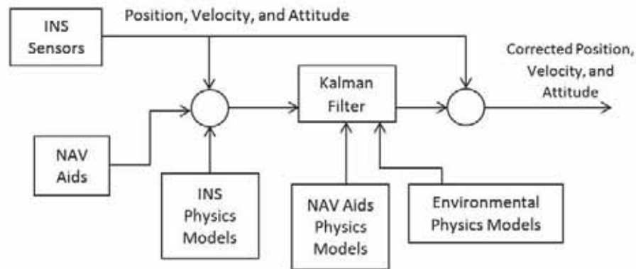
Figure 2022. Block diagram of Kalman Filter inputs.
