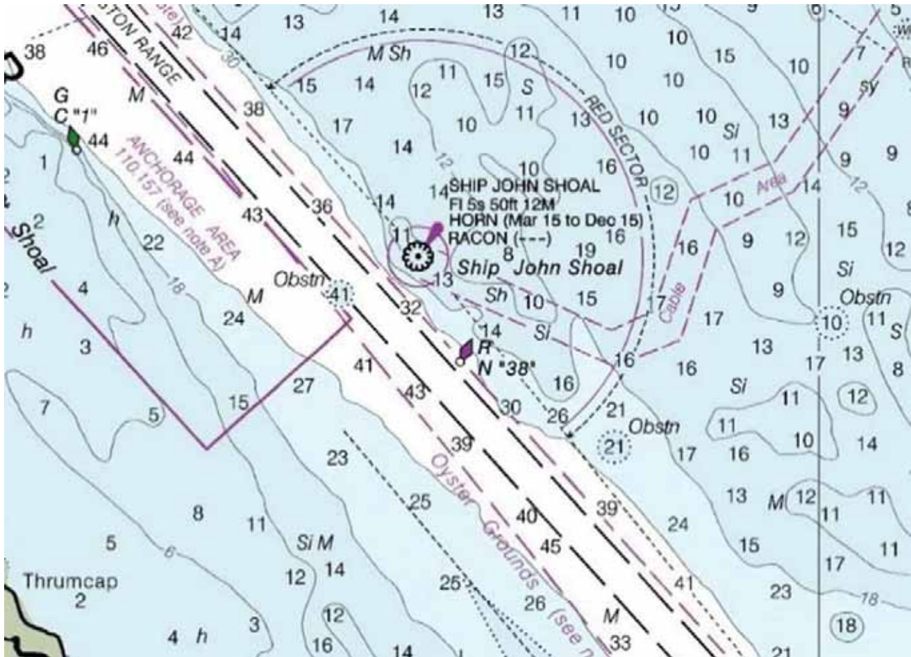
Figure 719. Portion of a chart depicting a light sector.
