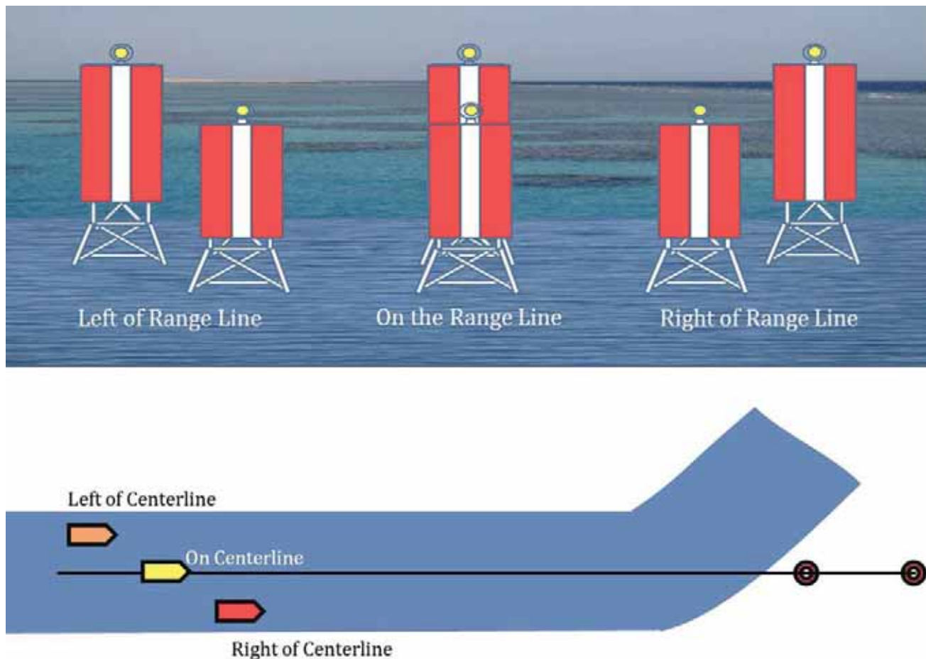
Figure 713. Example of Range Light aspects.
