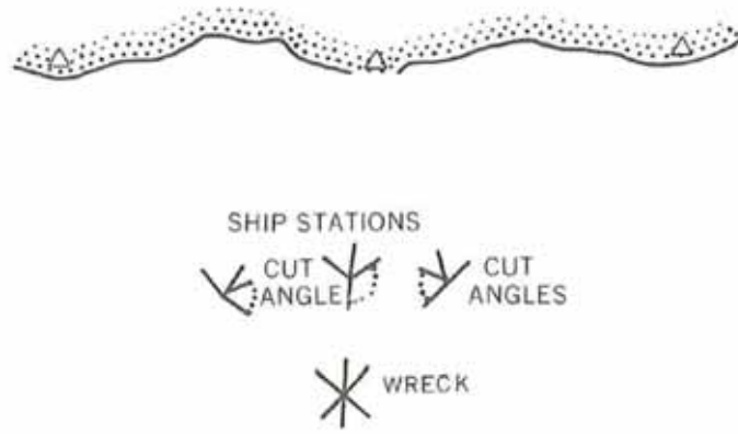
Figure 1107b. Cutting in uncharted objects.
