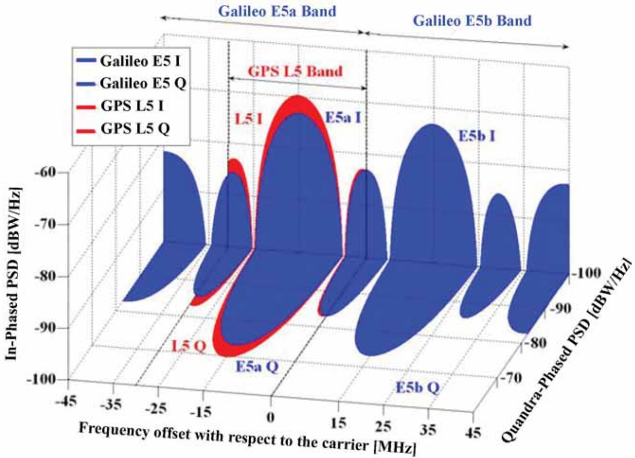
Figure 006c. Spectra of GPS and Galileo Signals in E5. Image courtesy of Dr. Jose Angel Avila Rodriguez.
