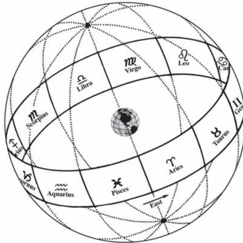
Figure 1321. The Zodiac.
