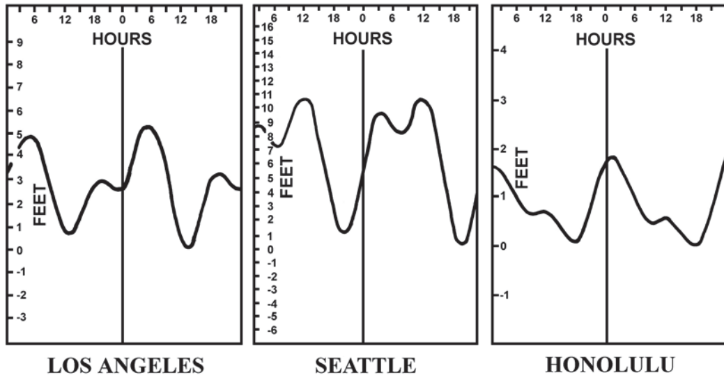
Figure 3505c. Mixed tide.
