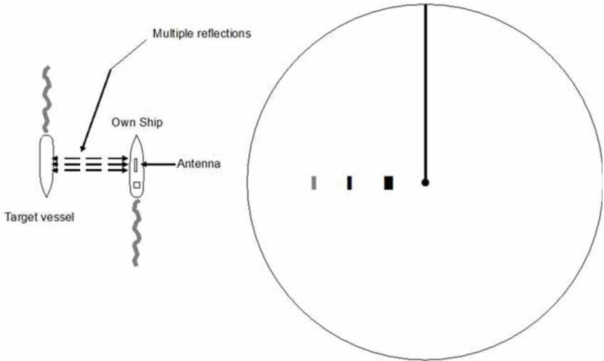
Figure 2310c. Multiple echoes.
