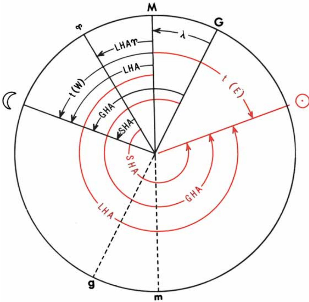
Figure 1326b. Time diagram.
